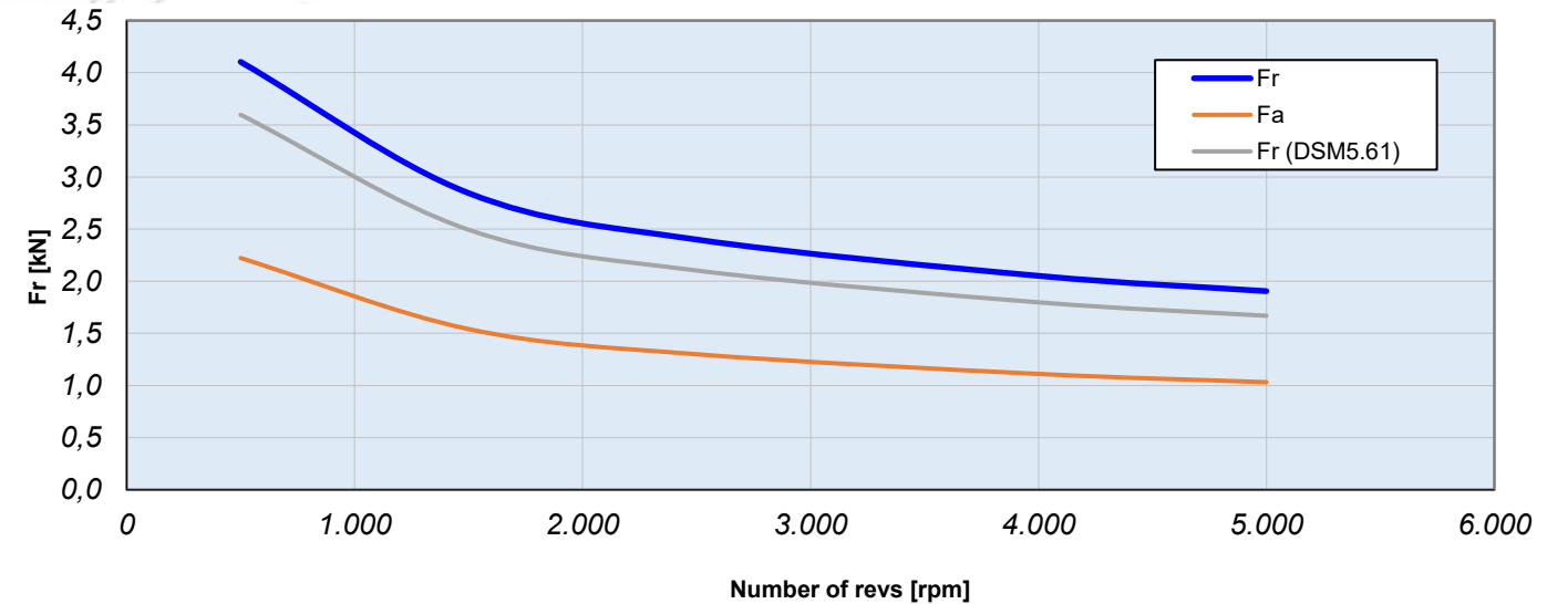
RADIAL & AXIAL SHAFT LOADING GRAPH
