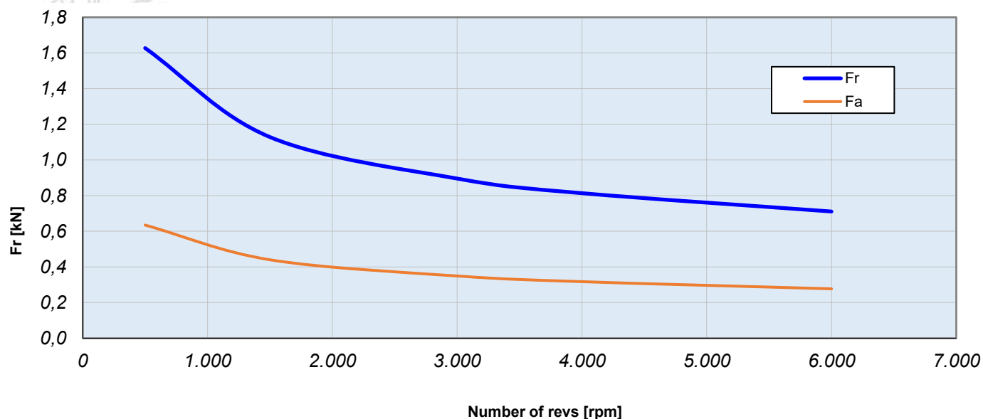
RADIAL & AXIAL SHAFT LOADING GRAPH
