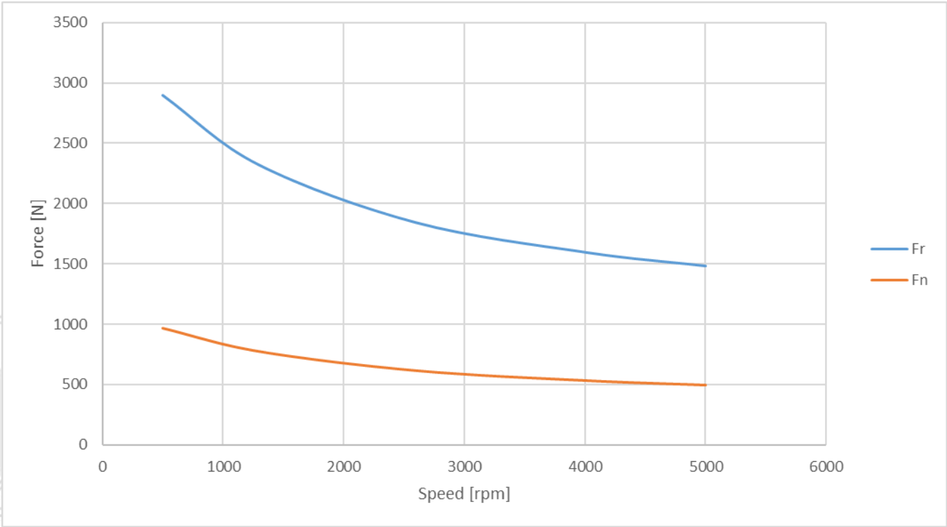
Frame 112 - RADIAL & AXIAL SHAFT LOADING GRAPH
