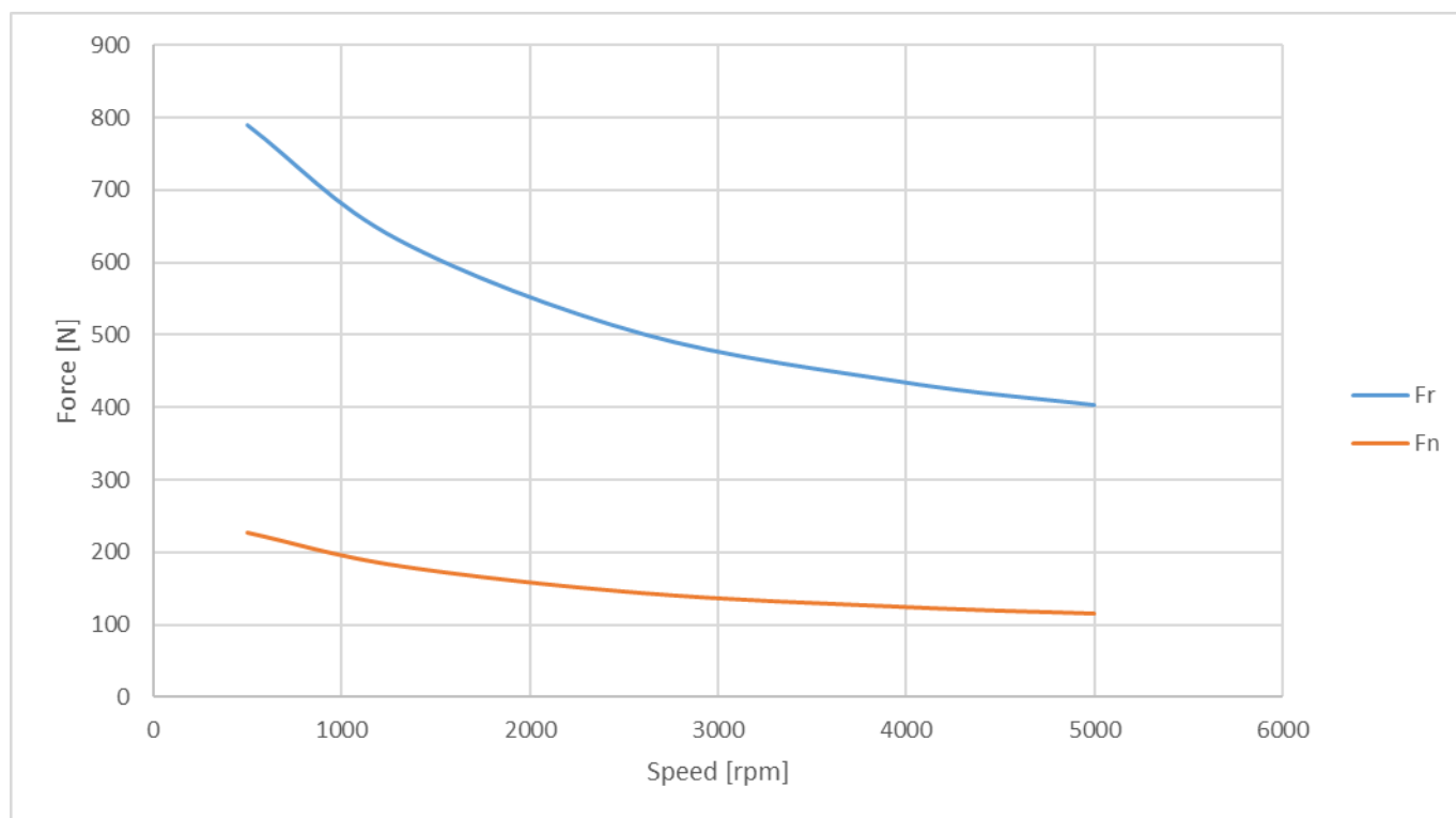
Frame 56 - RADIAL & AXIAL SHAFT LOADING GRAPH
