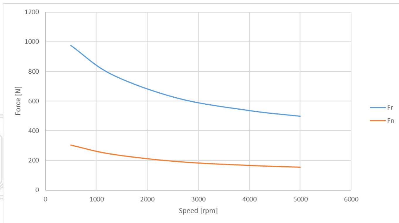
Frame 71 - RADIAL & AXIAL SHAFT LOADING GRAPH
