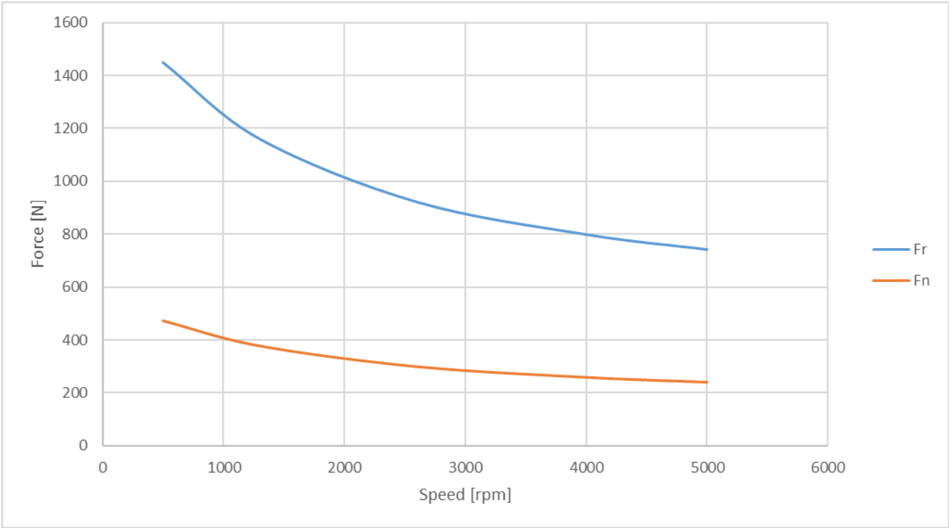
Frame 90 - RADIAL & AXIAL SHAFT LOADING GRAPH
