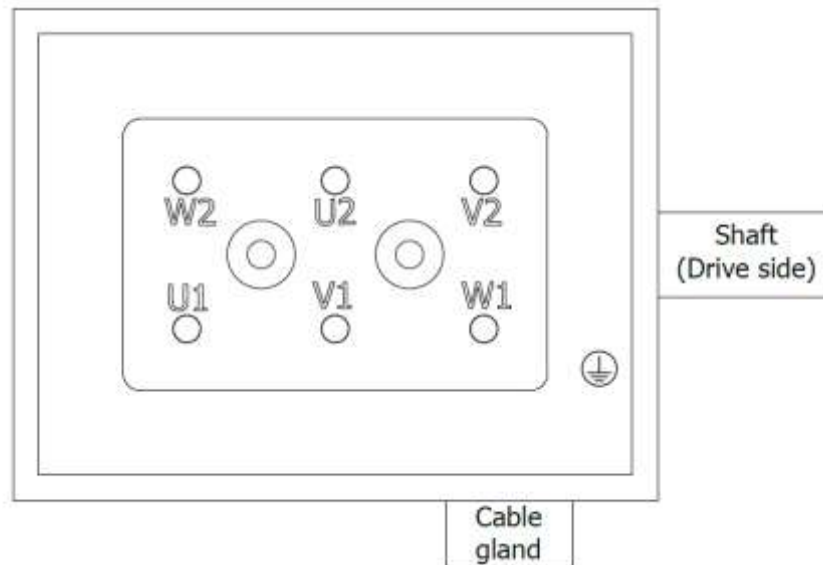
Motor terminal box top view
