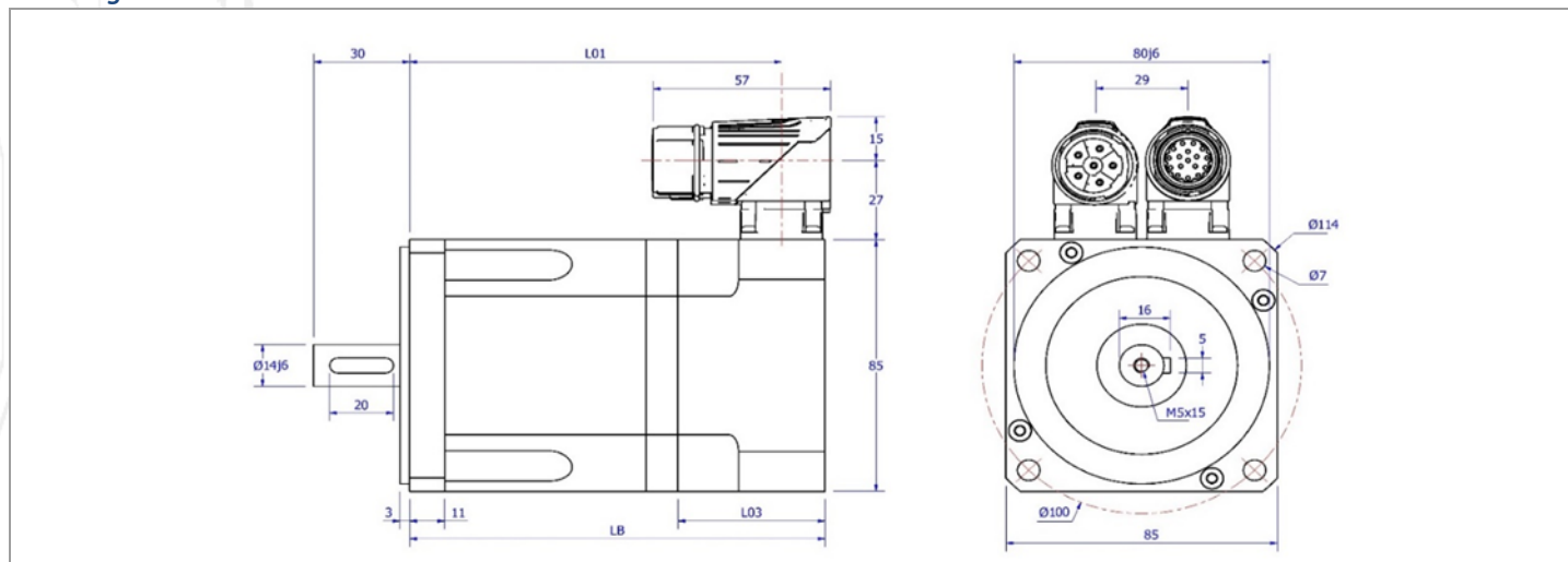
Dimension in mm
